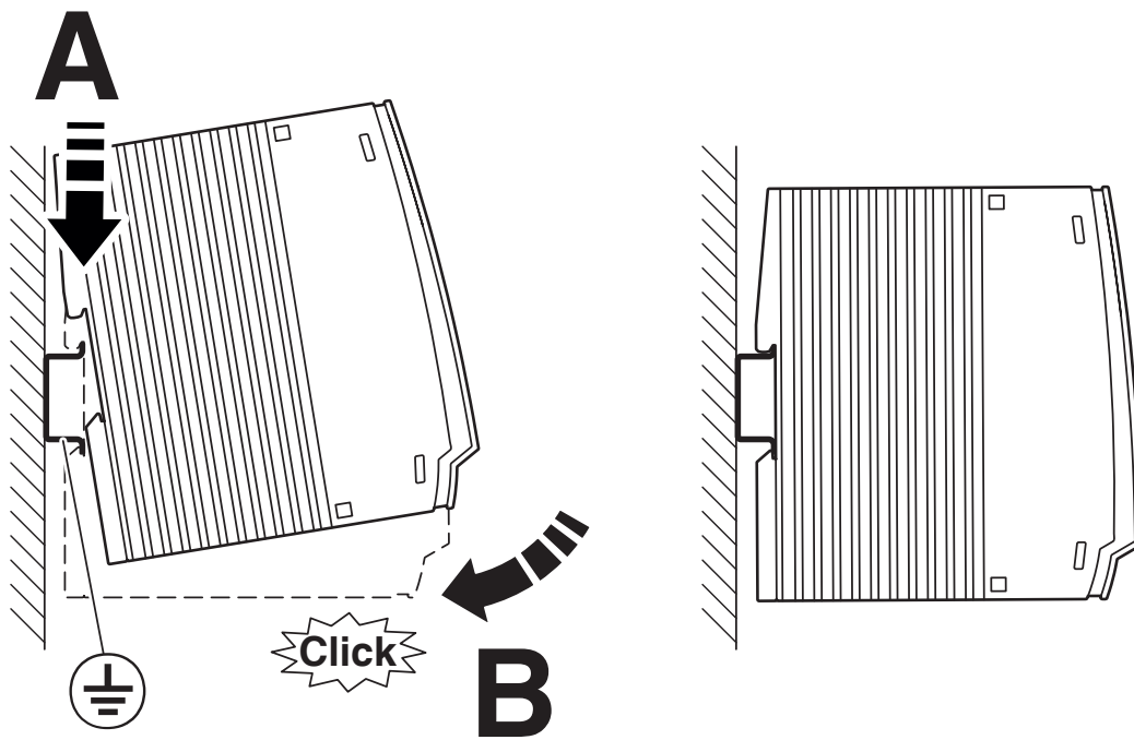
Schematic diagram
